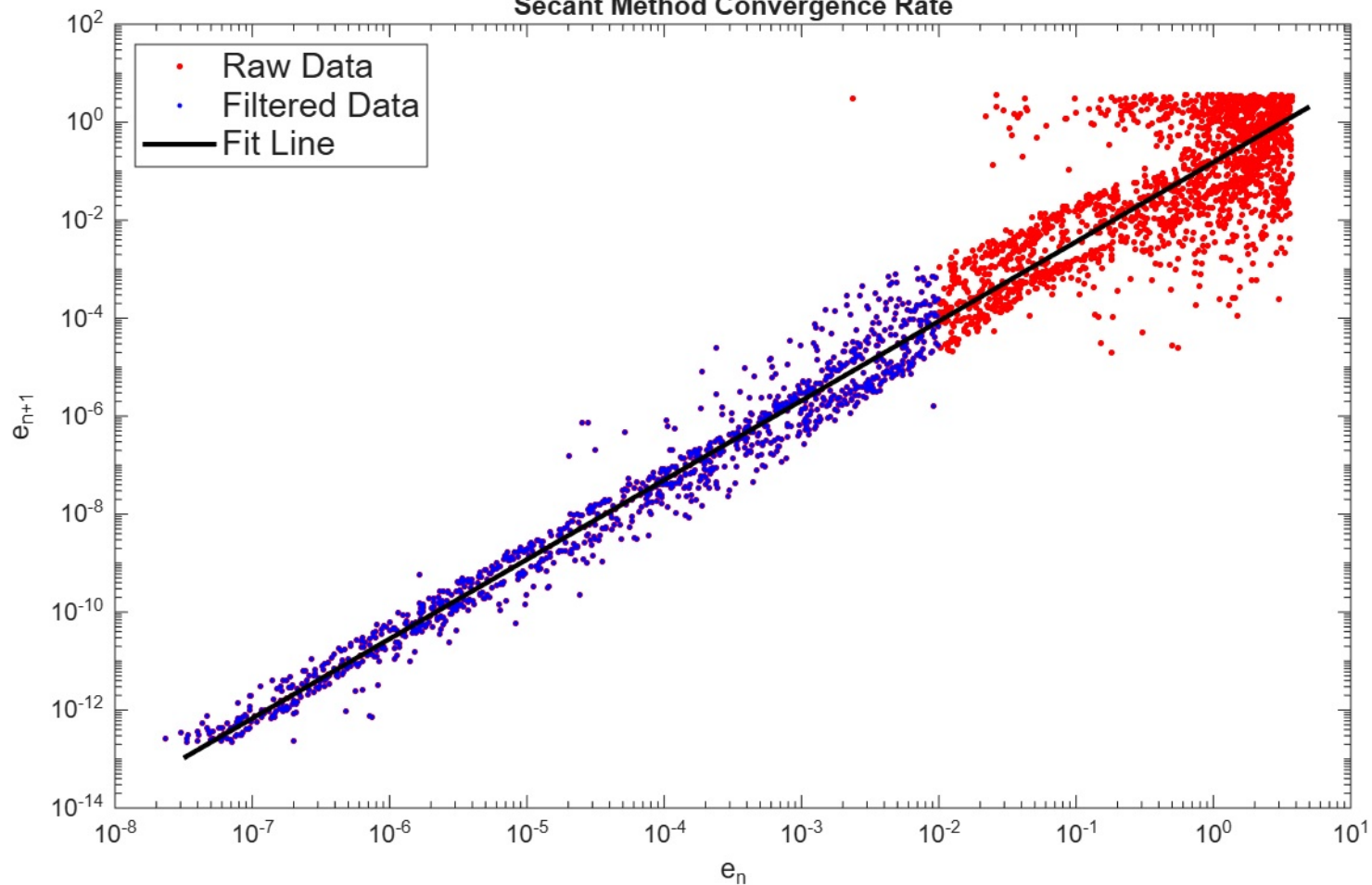
Secant Method Convergence Rate
